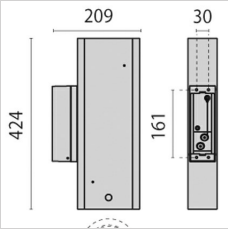
000442 Wall bracket 45
